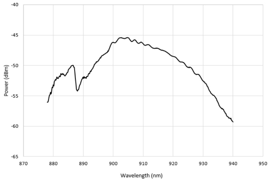
OEBS-100-920
